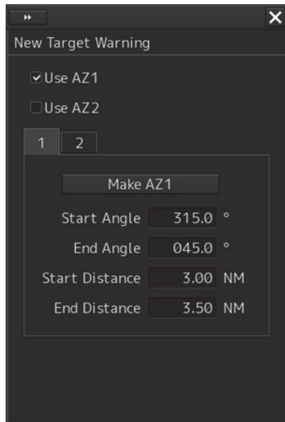
Settings of AZ1 (Automatic/Activation Area 1)
