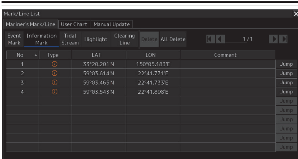
[Mariner's Mark/Line] tab (example at selection of [Information Mark])
