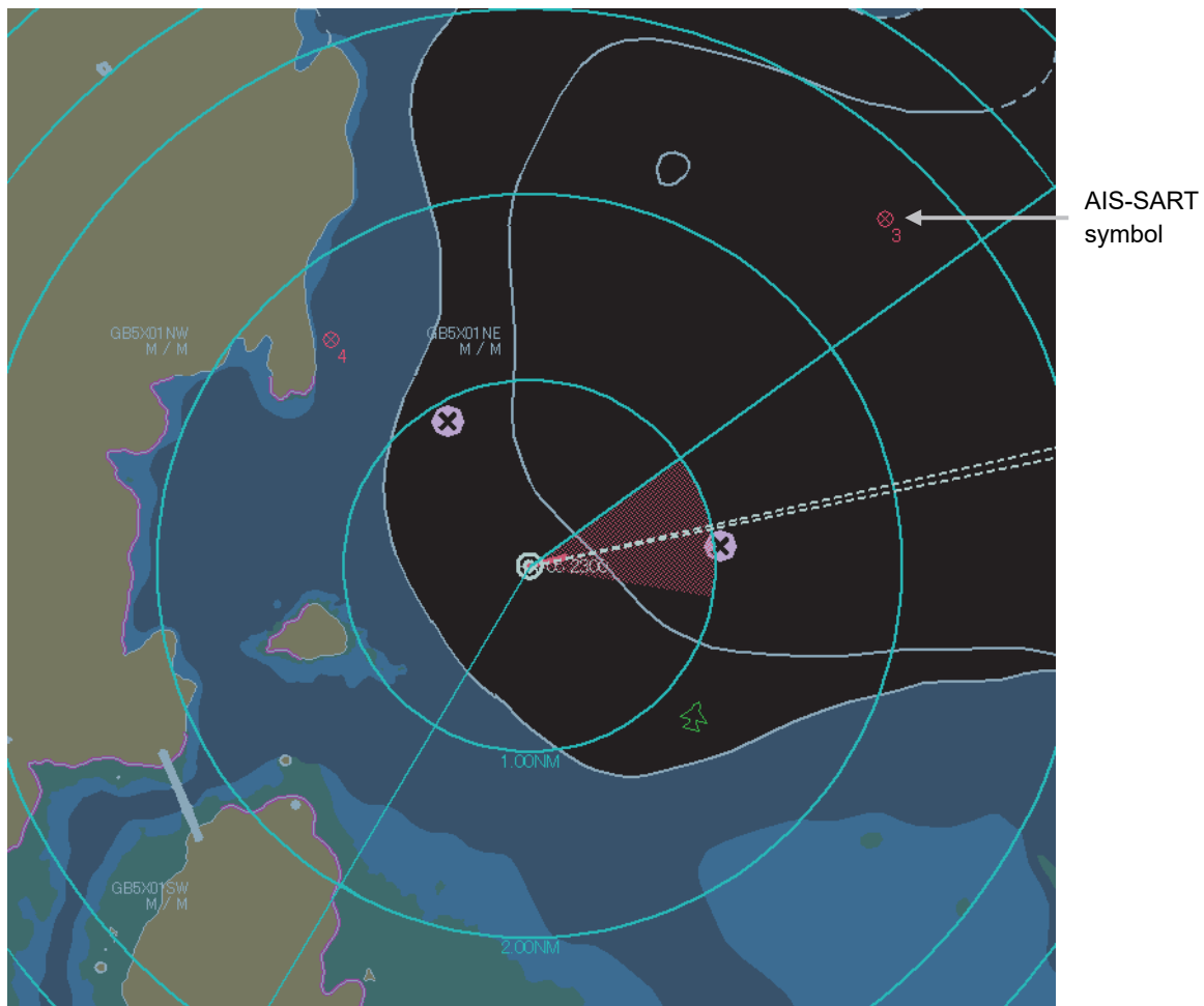
Example of AIS-SART Symbol Display
